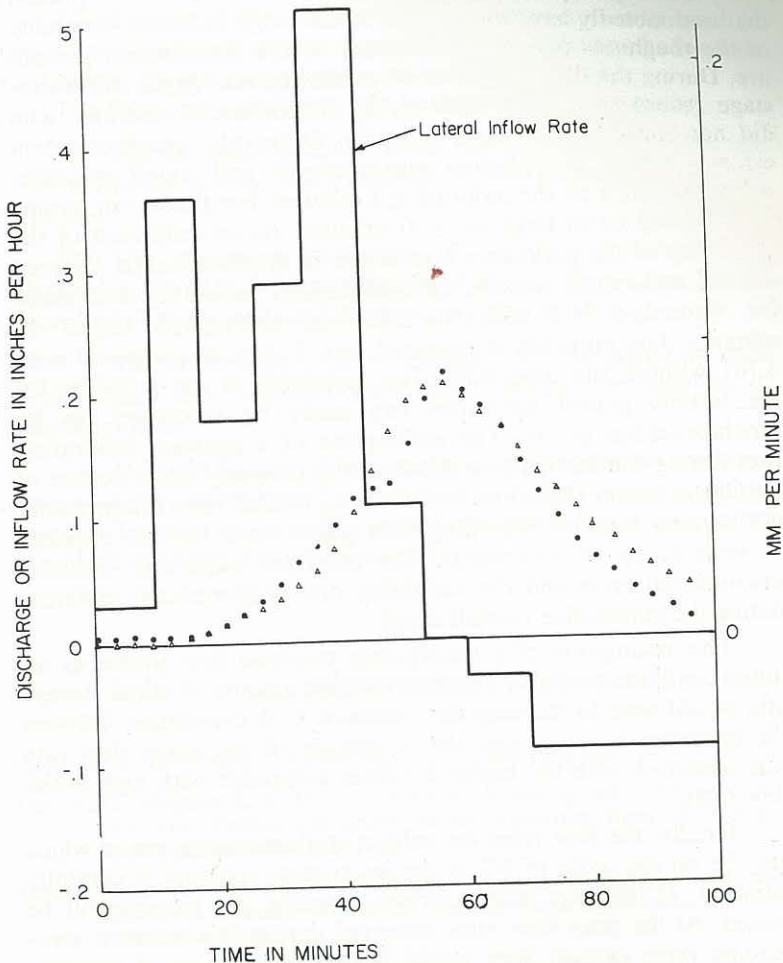
FIG. 9(b) — Best-fitting predicted hydrograph.
