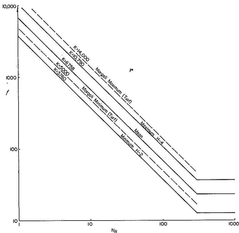
FIG. 8 — Darcy-Weisbach f versus Reynolds number.
