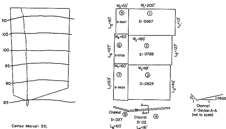
FIG. 5 — Topographic map and cascade representation of Watershed H-3, Cottonwood, South Dakota. (Scale, 1:2850.)
