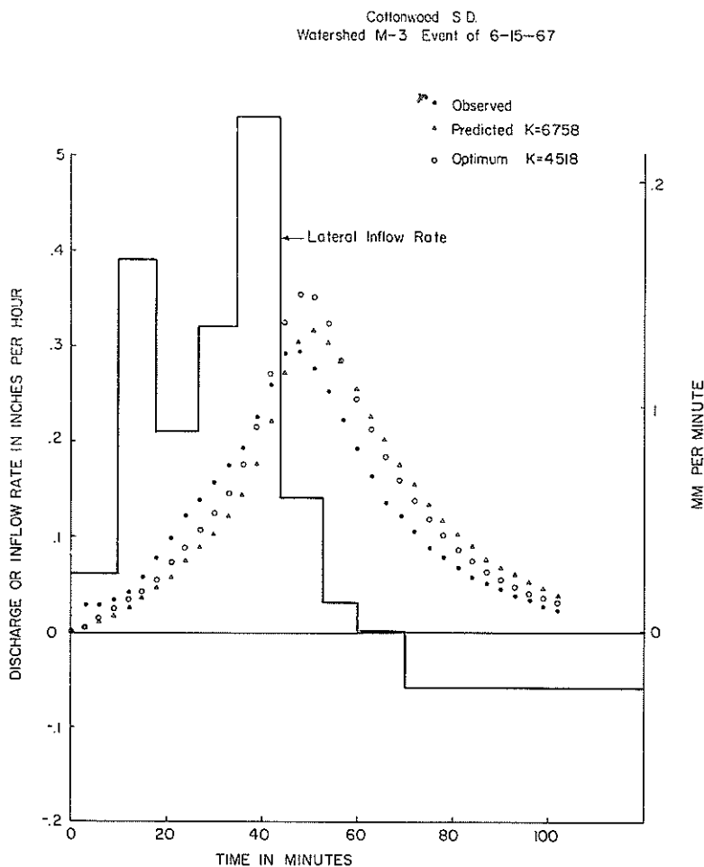
FIG. 9(a) — Worst-fitting predicted hydrograph.
