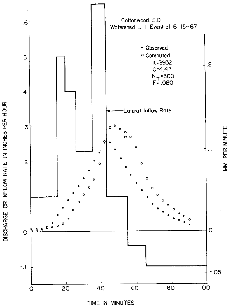
FIG. 7(a) — Worst-fitting optimized hydrograph.
