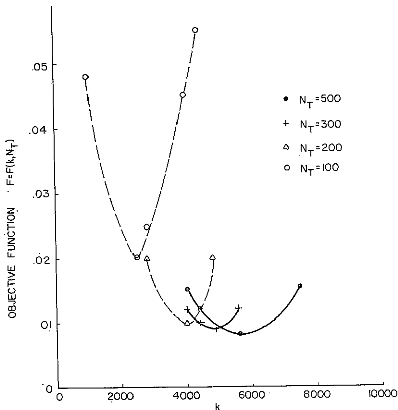
FIG. 6 — Objective function, Watershed H-1.
