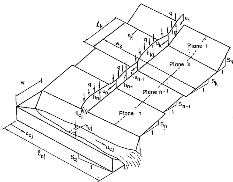
FIG. 1 — Cascade of n planes contributing lateral inflow to a channel.
