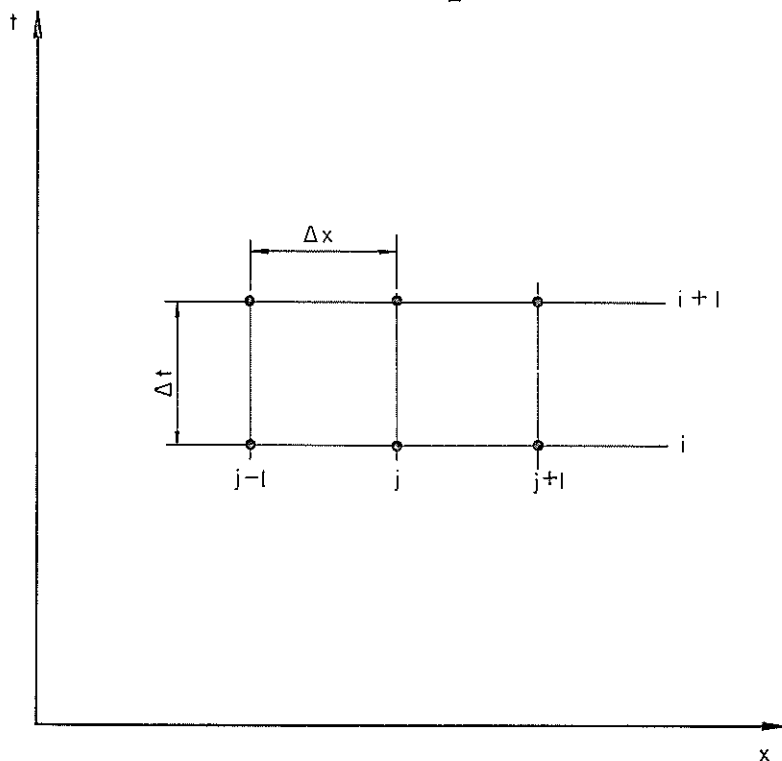
FIG. 2 — Notation for finite-difference schemes.
