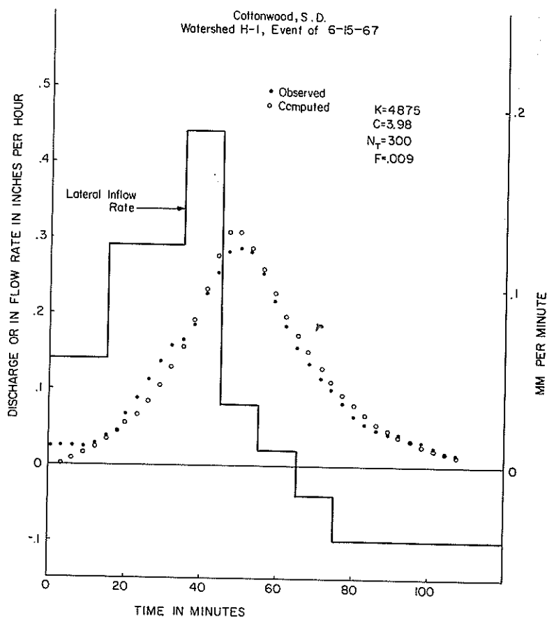
FIG. 7(b) — Best-fitting optimized hydrograph.
