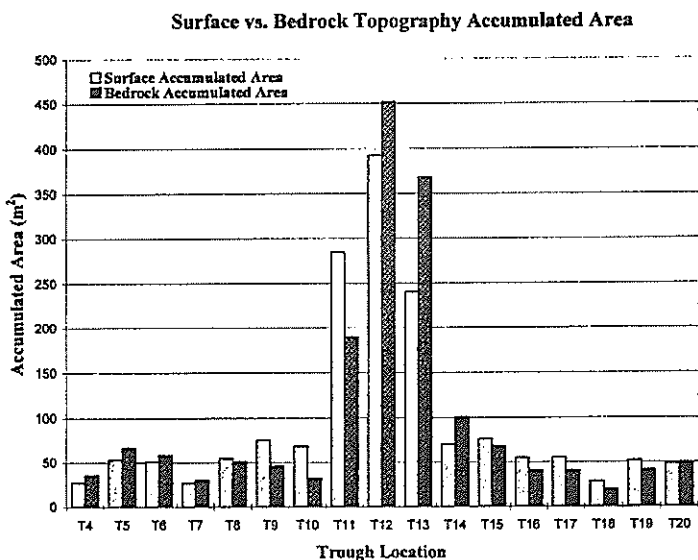
Figure 1 - Histogram plot of accumulated areas at the trough face for each section from the Woods and Rowe (1996) trench. The plot is based upon calculations developed by Freer et al. (1997) using surface topography and bedrock topography taken from a paper by Brammer et al. (1997) and data generously provided by Ross Woods. The result is a marked difference in the distribution at the trench face: there is a pronounced shift in accumulated area in the central trench portion to troughs 13 and 14 based on a bedrock surface calculation. This may explain the higher-than-expected contributions from trough 13 and some of the variability witnessed by Woods and Rowe (1996).
