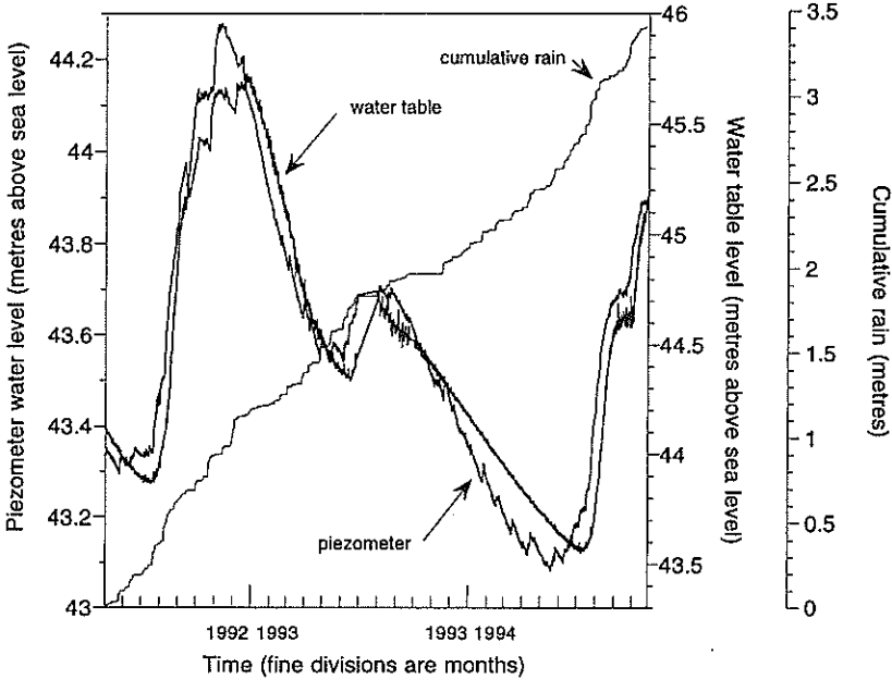
FIG 1 — Comparison of water table elevation and the piezometric head in a confined aquifer 40 metres beneath the surface, near Matamata, New Zealand. Water table elevations are data as recorded, the piezometric heads have been corrected for barometric pressure effects. The saw-tooth rises in the piezometer water levels are the loading impacts of individual rainfall events.
