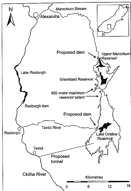
Figure 1 – The Onslow-Manorburn depression, showing maximum pumped storage reservoir development to 800 metre elevation in both Upper Manorburn and Lake Onslow basins.
