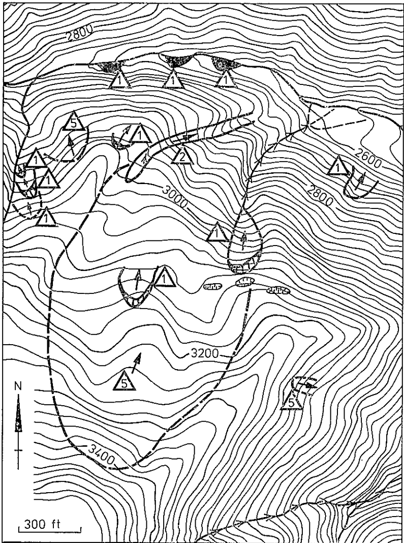
FIGURE 2—Landslide and influence area map: Scale 1 inch = 300 feet.
