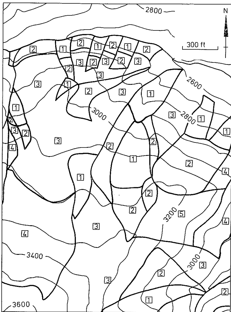
FIGURE 3—Hazard zonation map.
